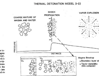
Fig. 5. An alternative model of strong magma-water interaction. Following by explosion requires the propagation and maintenance of a shock wave as a thermal detonation. The inset first shows an expanded view of conditions across the shock wave where u_1 is the shock velocity, u_2 is the water velocity, and u_3 is the magma fragment velocity. Where u_2 > u_3 , a large enough magmatic magma breakup by processes such as boundary layer stripping and Taylor instability may result in large fast moving debris.
