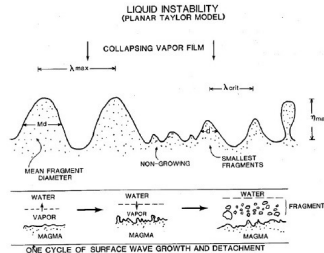
Fig. 4. Illustration of a planar Taylor instability at the interface between magma and a collapsing water-vapor film (top). A complete cycle of instability growth is shown at the bottom (see text for description). Oscillation of the film thickness requires sufficient momentum in the magma so that its surface distorts into waves that can grow until they detach to form small fragments.
