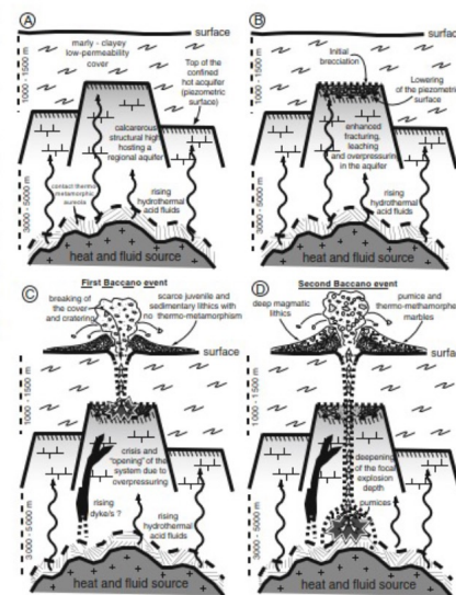
Fig. 4 Model for type 1 phreatic systems and eruptions. A shallow magma body releases gas by intrusion and/or crystallization. The gases are transported upward through a series of cracks, intersecting the hydrothermal system above. If the hydrothermal system is sealed at its top, the system will become pressurized from the addition of hot magmatic gases. Such conditions promote phreatic eruptions
